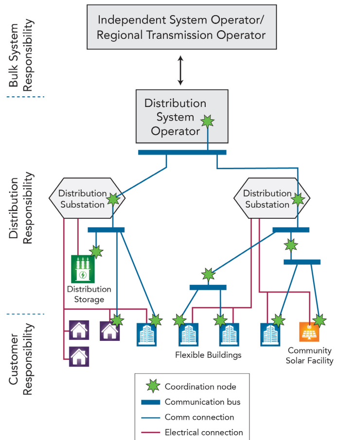
Figure 5. Utility Architecture View with Layered Decomposition Coordination
