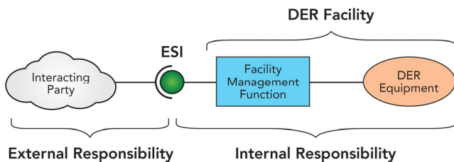
Figure 6. Components of DER and Grid Integration
